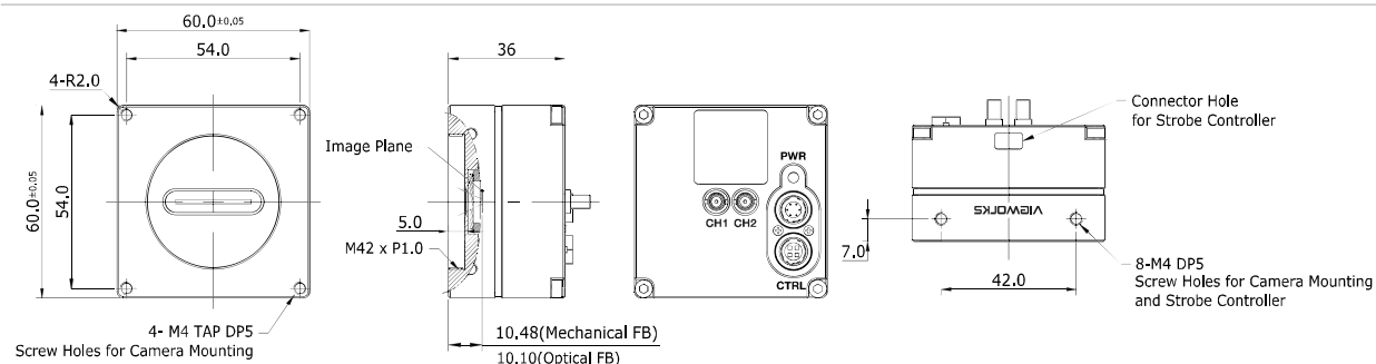
Mechanical Dimension in mm
